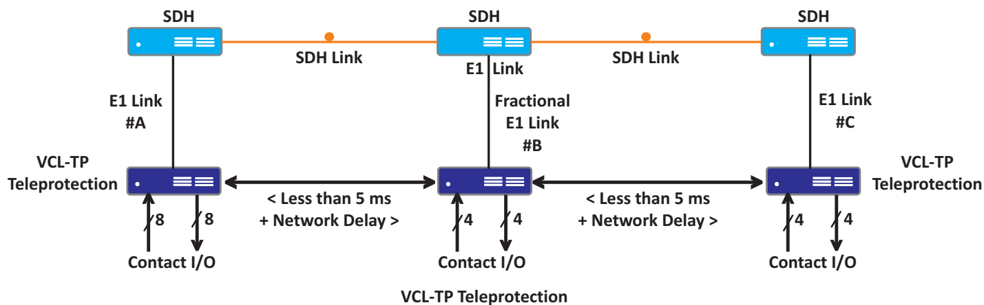
E1 (2.048Mbps) transmission link in an add-drop application - 4 x Binary Commands to Site # B and 4 Binary Commands to Site # C
