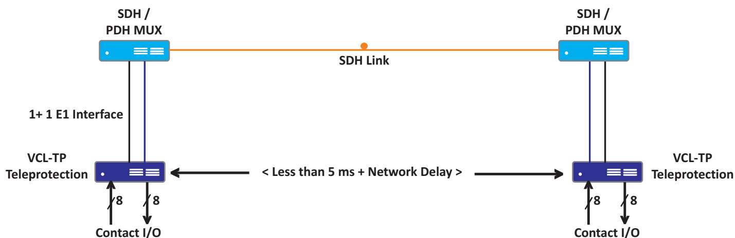
1+1 Redundant E1 interface with link failure detection and automatic failover
