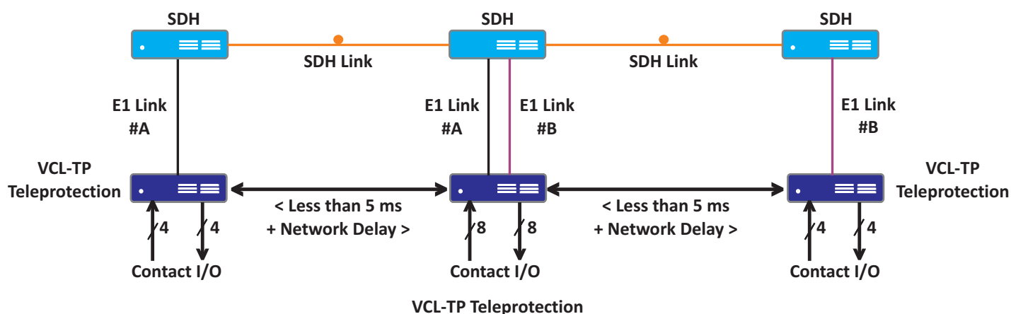
E1 (2.048Mbps) transmission link in a point-to-multipoint application 4 Binary Commands on E1 Link # A and 4 Binary Commands on E1 Link # B
